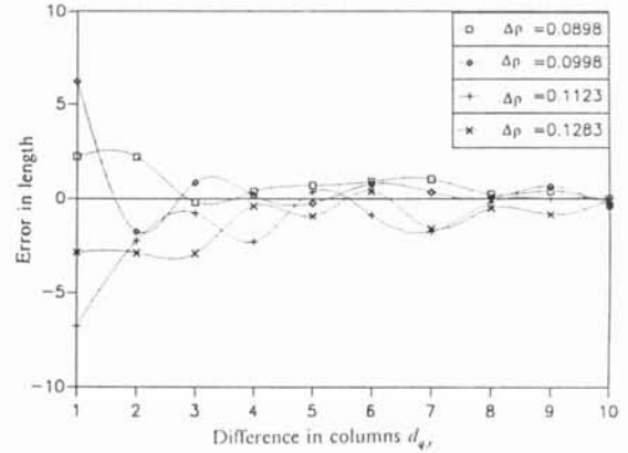
Figure 4: Errors in the line length vs. d_{q,r} for a line having \rho_a = 90 and \theta_a = 25^\circ .
